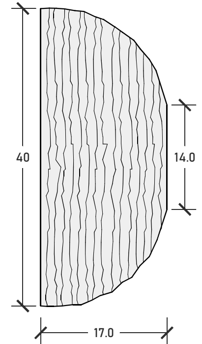
Fianco | Side
