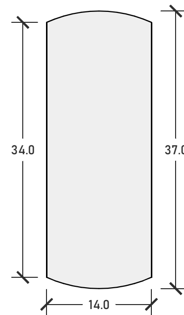
Fianco | Side
