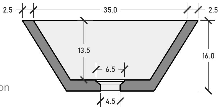
Fianco | Side
