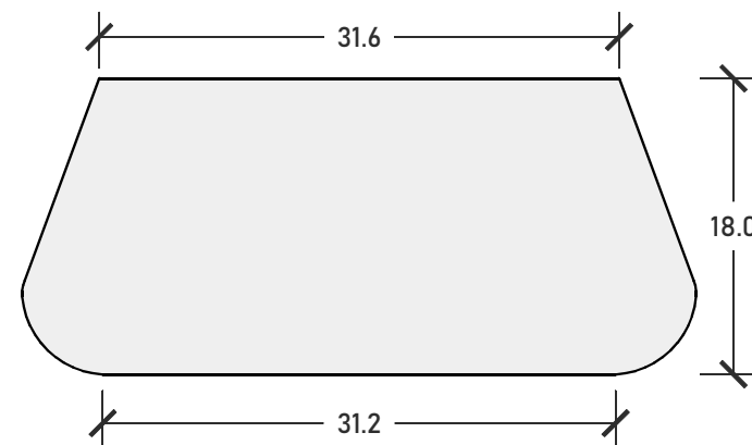
Fianco | Side
