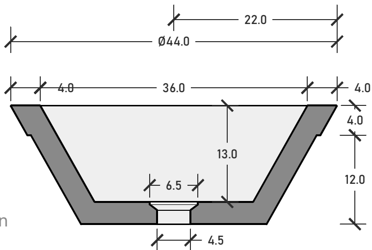
Fianco | Side
